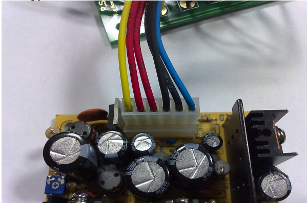
Yellow (12V), Red, Red (5V), Black, Black (0V), Blue (-12V).
