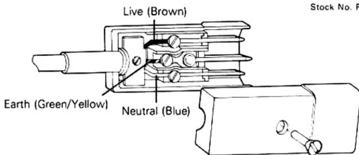
Fig. 2 A.C. Output Connector CEE22 cable ended plug.
