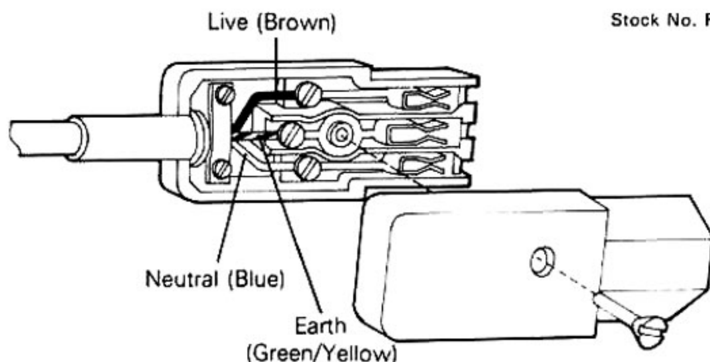
Fig. 1 A.C. Input Connector CEE22 cable ended socket.
