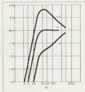
Fixed low frequency filter (at limits of bass control settings)
