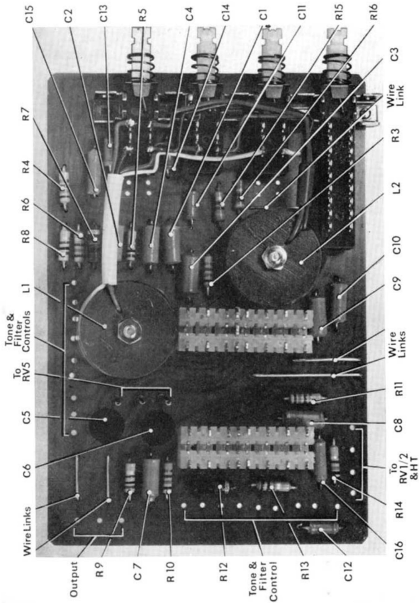
Fig. 8 Filter Board M.12029
