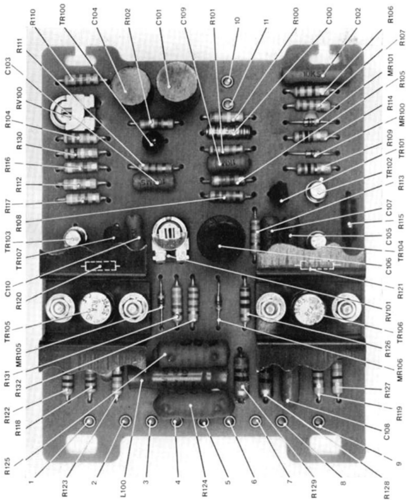
Fig. 11 (b) Driver Board M.12038 (issue 10)
