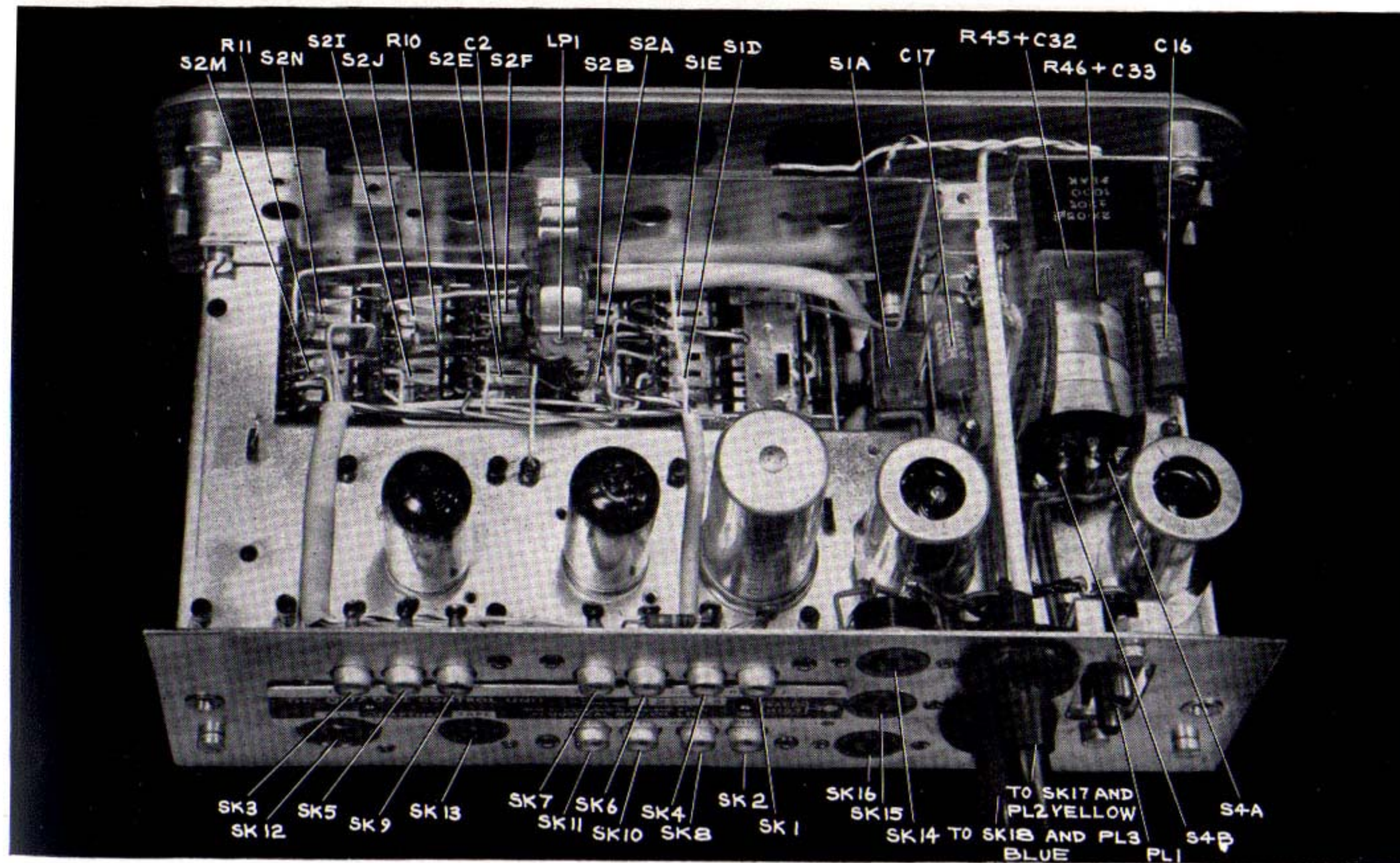
LAYOUT PHOTOGRAPH C
