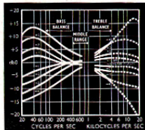
Curves showing extended frequency response and effect of the 7K filters.
