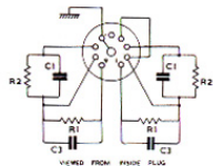
SINGLE LETTER ADAPTOR
