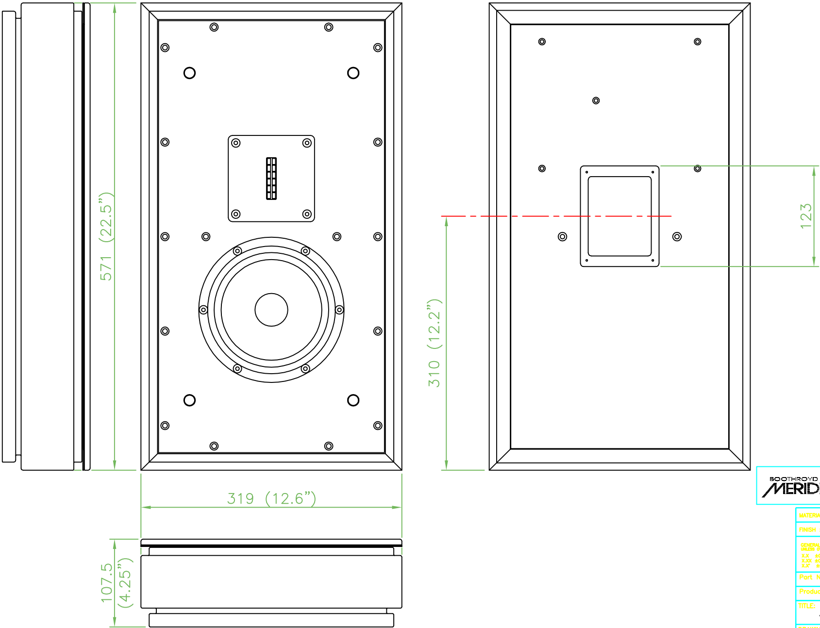
FRONT VIEW DRAWN WITH GRILLE REMOVED FOR CLARITY
