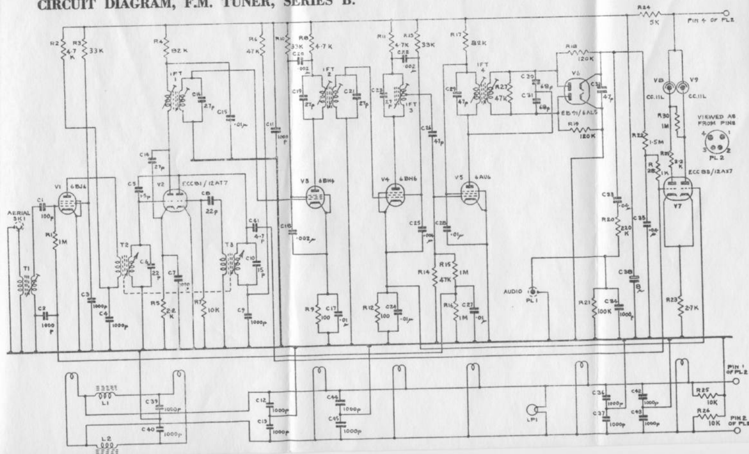
CIRCUIT DIAGRAM, F.M. TUNER, SERIES B.
