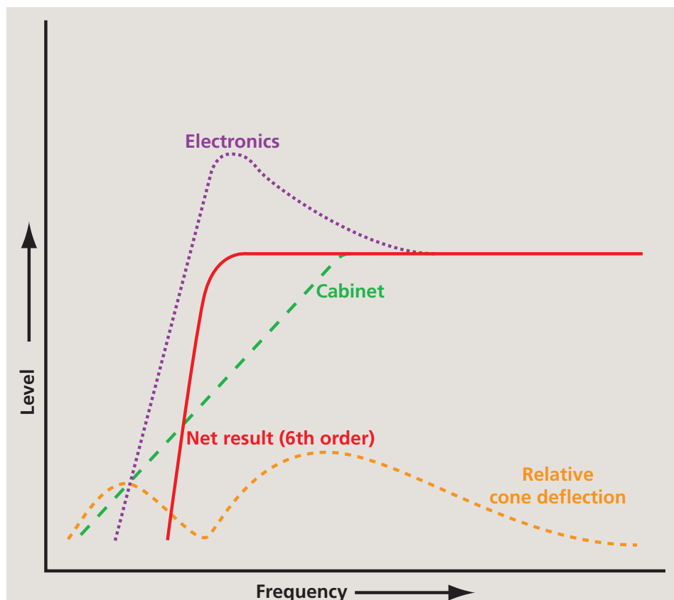
Fig. 4: The overall response of an active speaker can be tailored, the bass improved and the maximum cone excursion limited by careful use of electronic filters.
