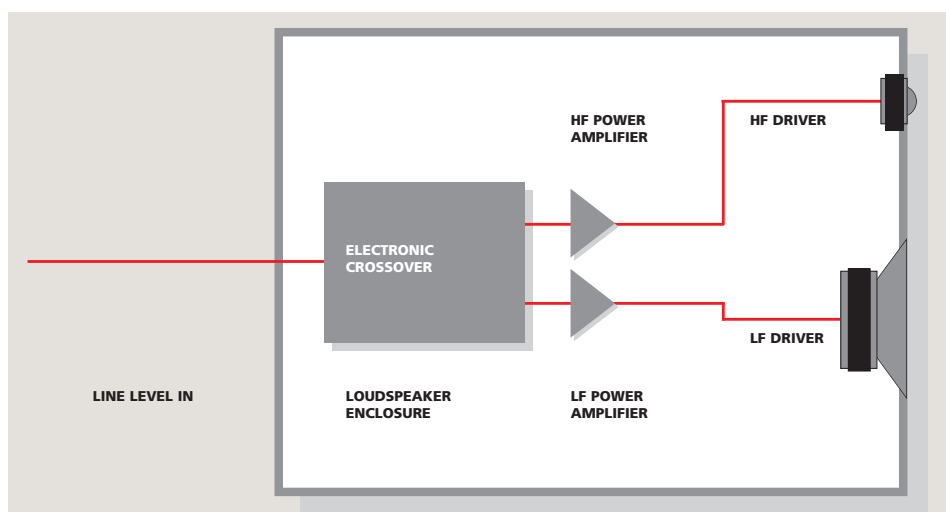
Fig. 2: An alternative arrangement to that shown in Figure 1, in which an electronic, line-level crossover drives a pair of amplifiers feeding woofer and tweeter.
