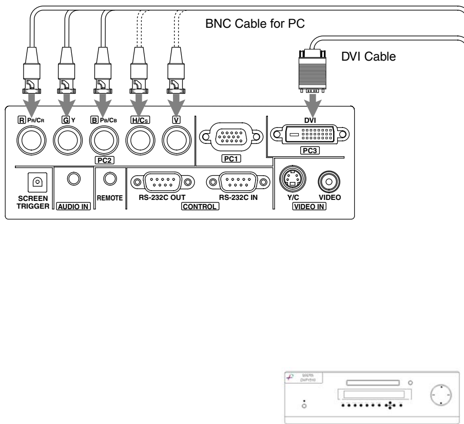
■ Video Processor
