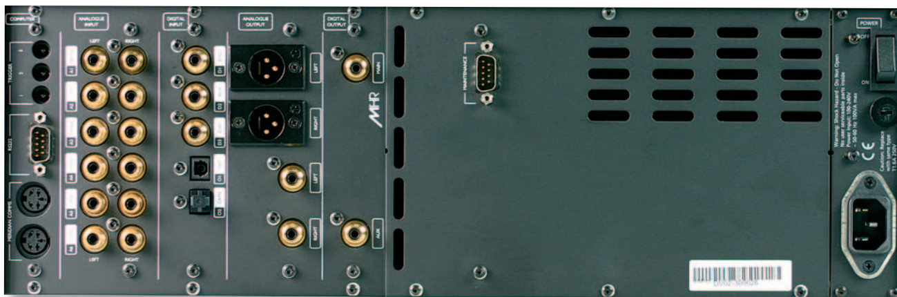
808i (Player/Preamplifier model) Rear Panel. The 808 Player model does not include the analogue and digital input panel areas.
